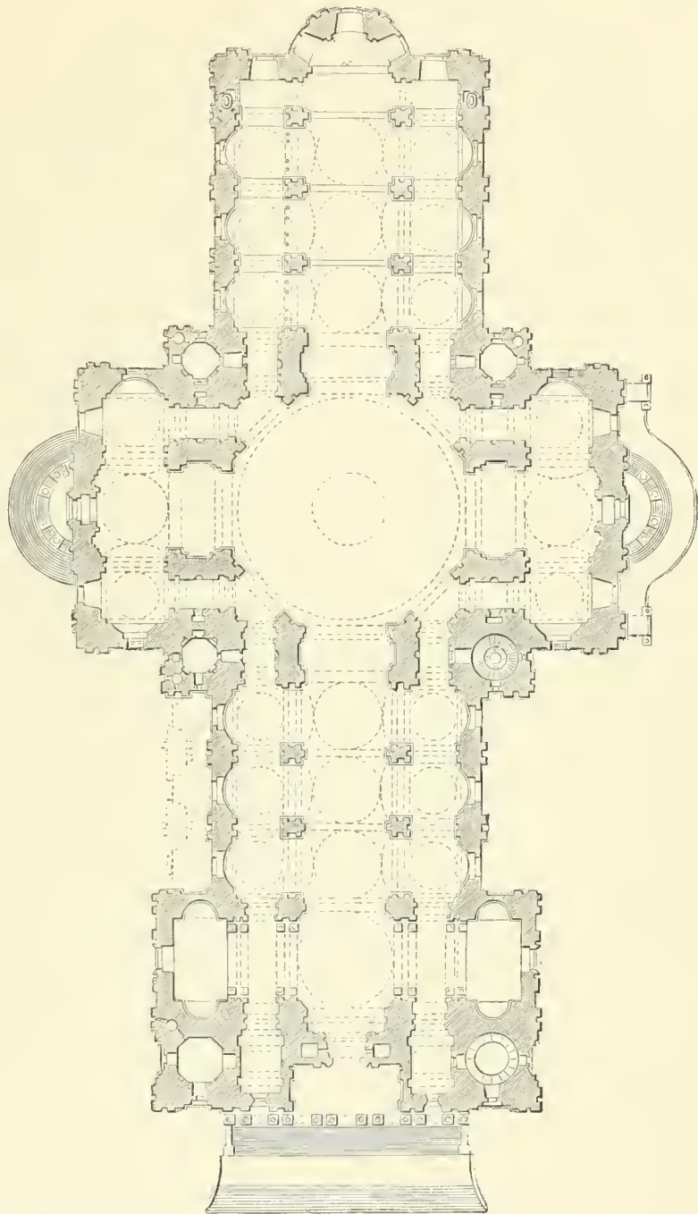
PLAN OF ST. PAUL'S. 1
